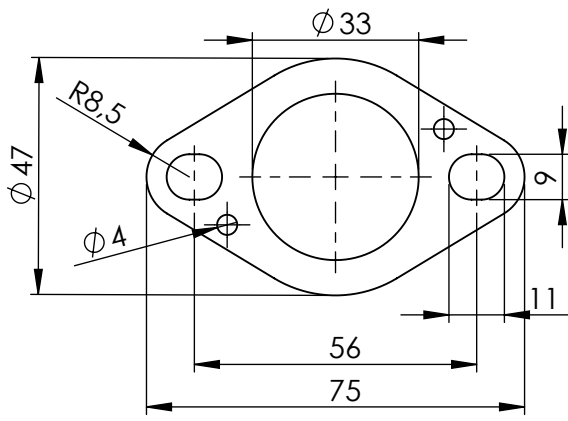
S.s. Flange "45E" cod.205267 sp.6mm
