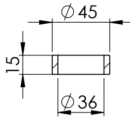
S.S. Bushing P/N 207133
