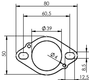
S.S. Flange 158A sp. 6mm P/N 206061
