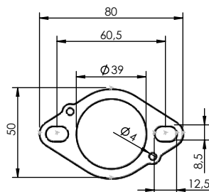
S.S. Flange 158A sp. 6mm P/N 206061
