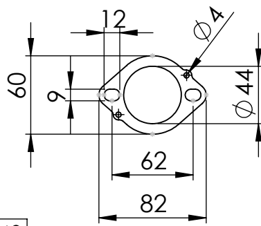
S.S. Flange 112A P/N 204569 sp.5mm
