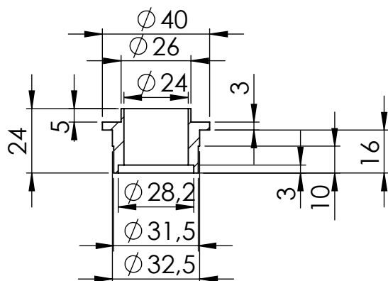
Bushing titanium cod.206634
