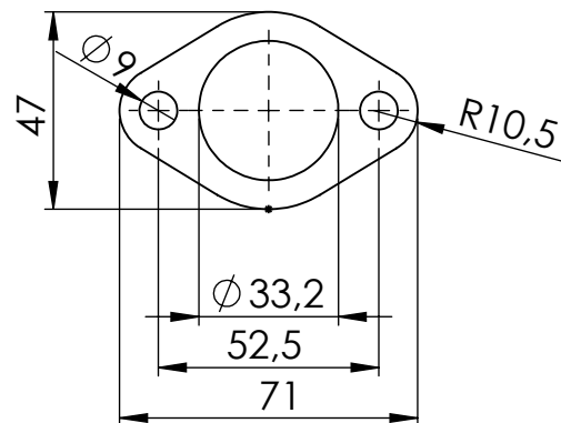
Flange 43T titanium sp.5mm cod.206641
