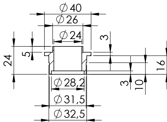
Bushing s.s cod.204640
