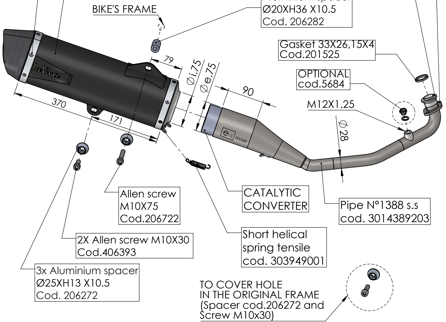
NERO silencer RHS stainless steel black Cod.3014081481
