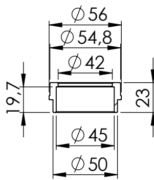
s.s. bushing cod.206424
