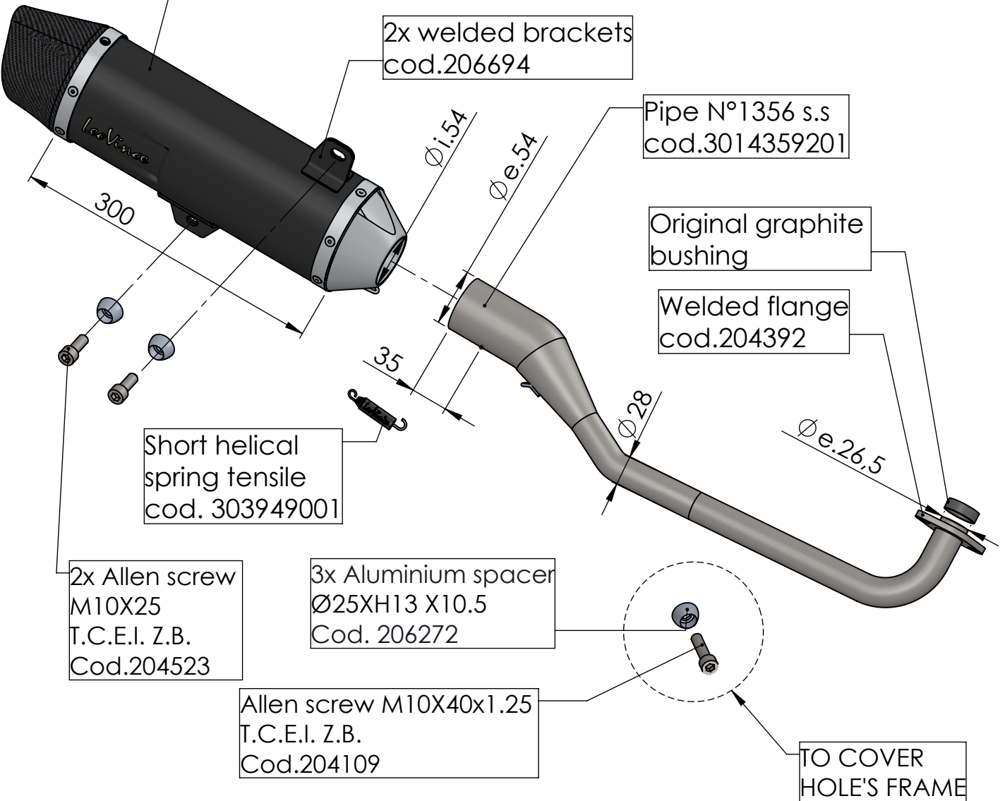
NERO silencer RHS stainless steel Cod.3014070481
