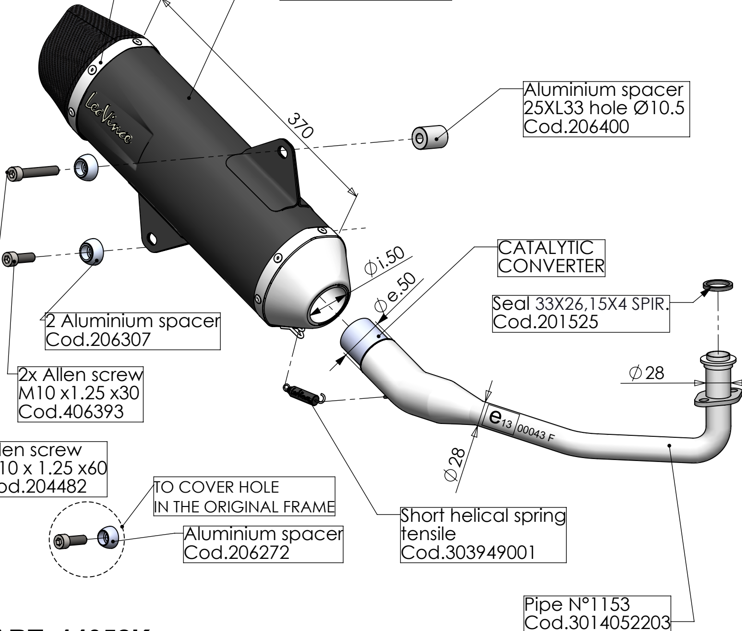
NERO silencer stainless steel black Cod.3014052471
