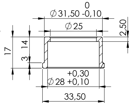
S.s cylinder bushing cod.206539
