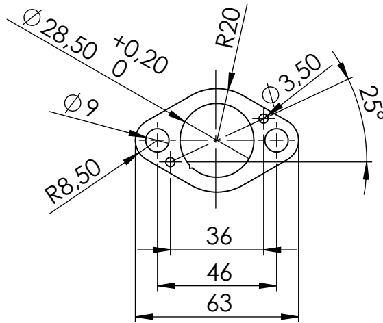
S.s flange sp. 6mm cod.206538
