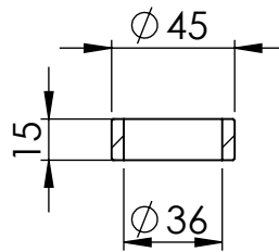
S.S. Bushing P/N 207133
