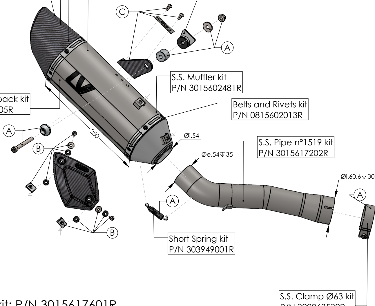
Outer Sleeve kit P/N 3015602010LR
