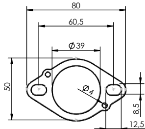
S.S. Flange 158A kit sp. 6mm P/N 206061R
