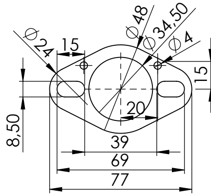
S.s. flange sp.5mm Cod.206443R
