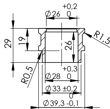
S.s. Bushing Cod.206442R
