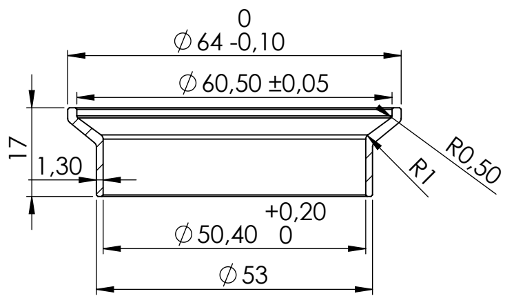
Bushing S.s. cod.206079
