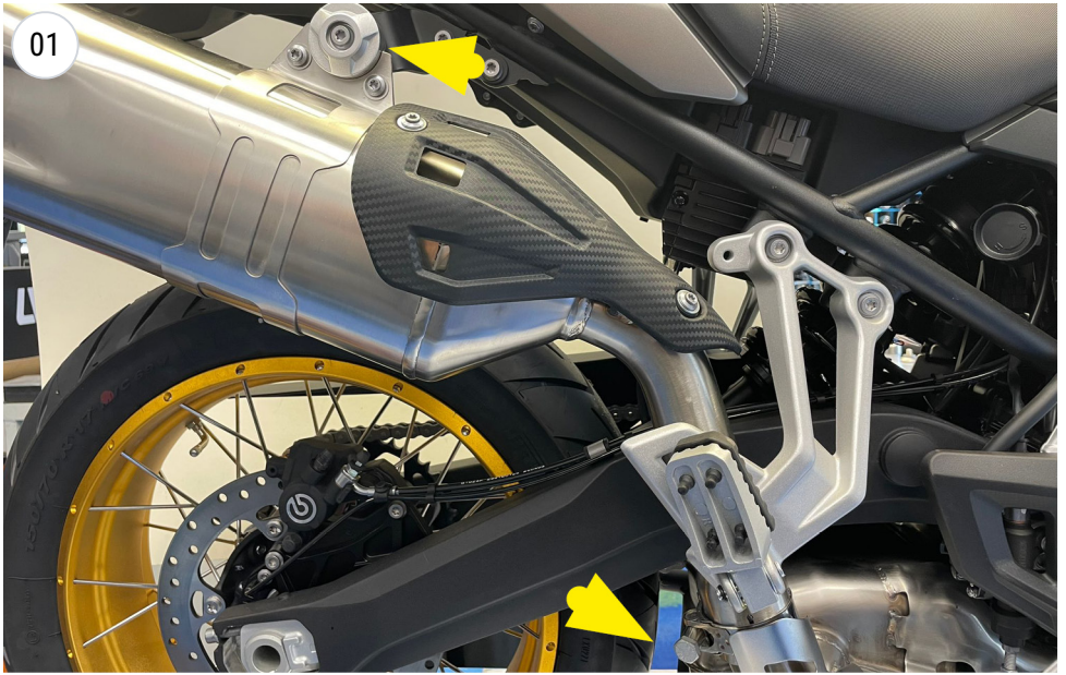
unscrew and remove the muffer
