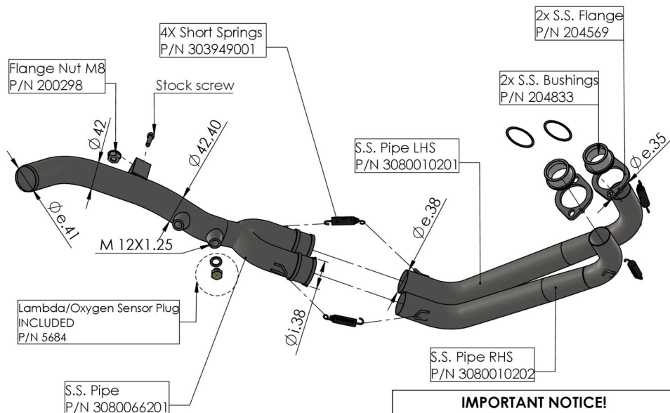
Bushing P/N 204833
