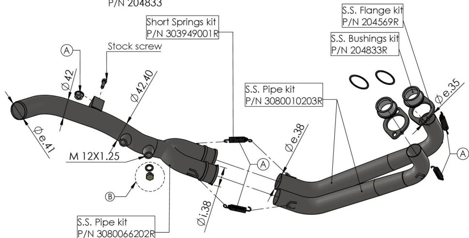
Bushing P/N 204833
