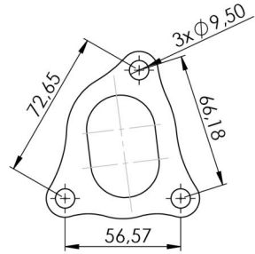
S.S. Flange 160A P/N 206084 sp.8 mm
