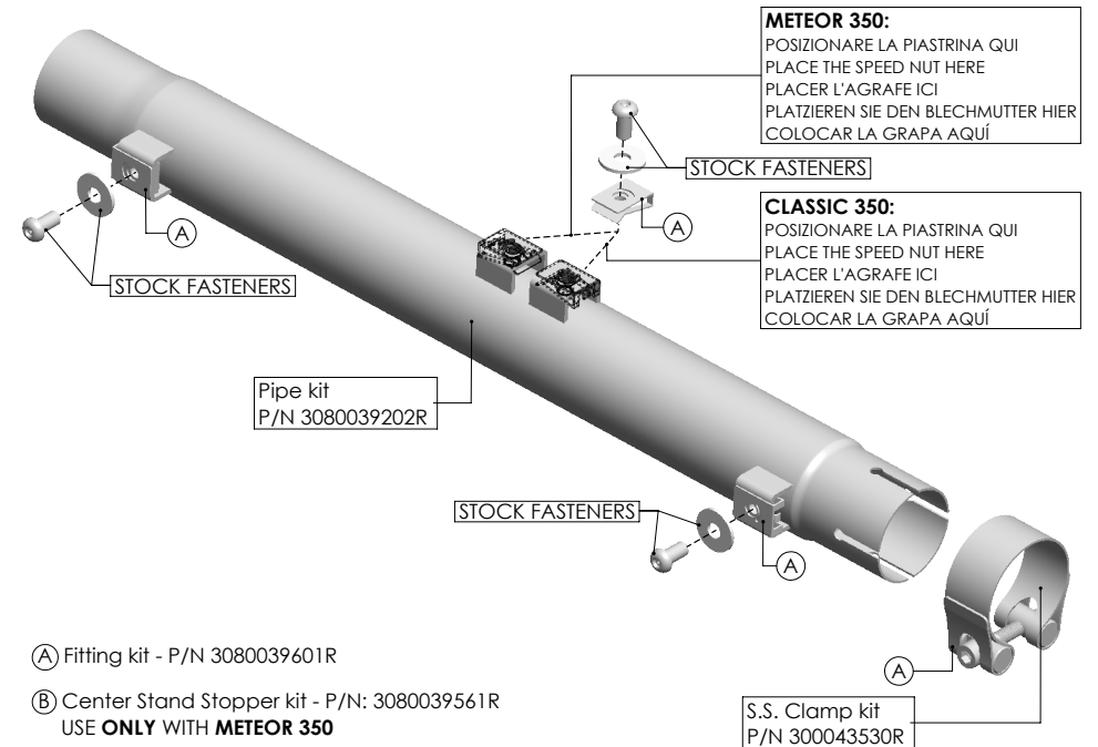
(B) Center Stand Stopper kit - P/N: 3080039561R USE ONLY WITH METEOR 350
