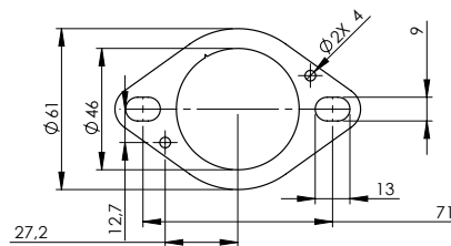
Flange s.s. sp.5mm cod.206412
