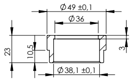
Bushing s.s. cod.206697
