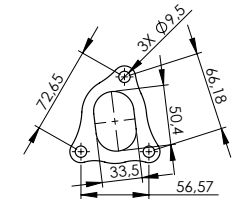
Flange "160A" cod.206084 sp.8mm
