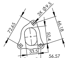
Flange "160A" cod.206084 sp.8mm
