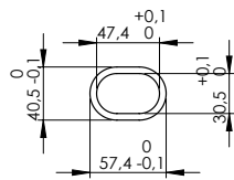
Bushing sp.8mm cod.206083
