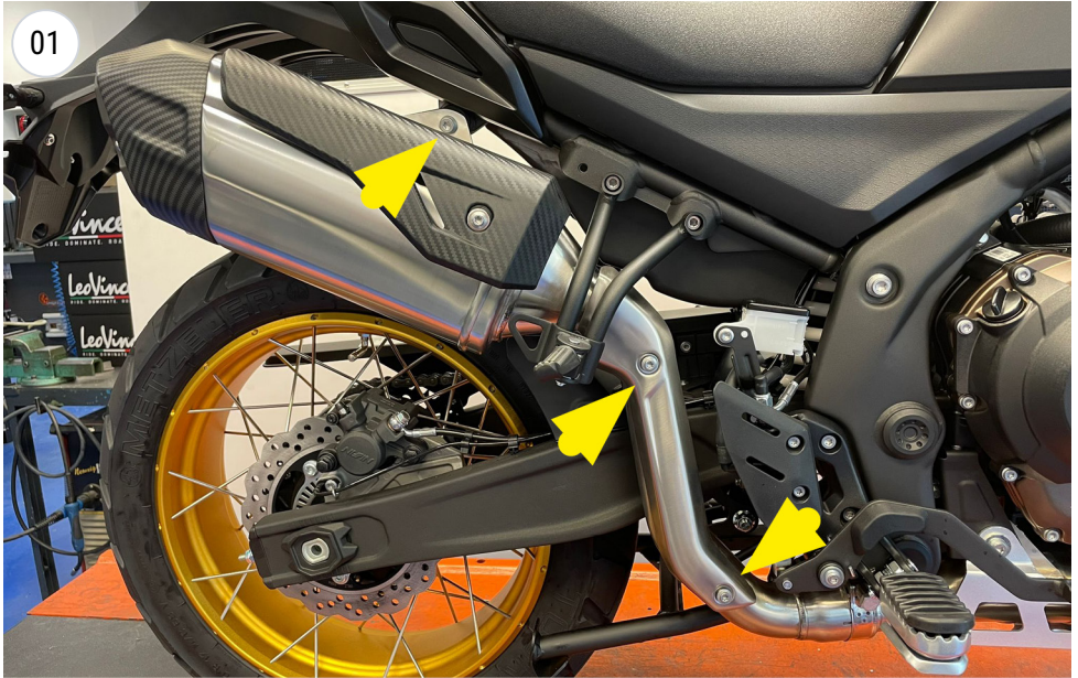
unscrew and remove the heat shield and the muffler
