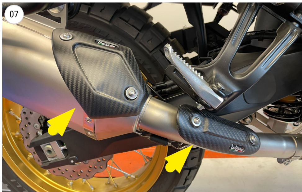
fit the carbon heat shields
