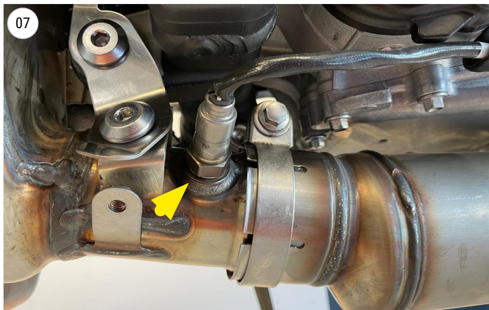
unscrew the Sonda lambda/O2 sensor
