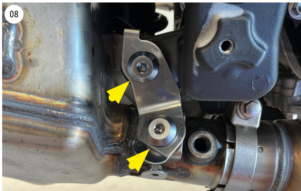
unscrew and remove the bracket
