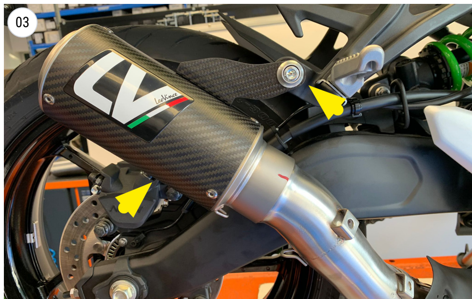
INSTALL THE LEOVINCE MUFFLER
