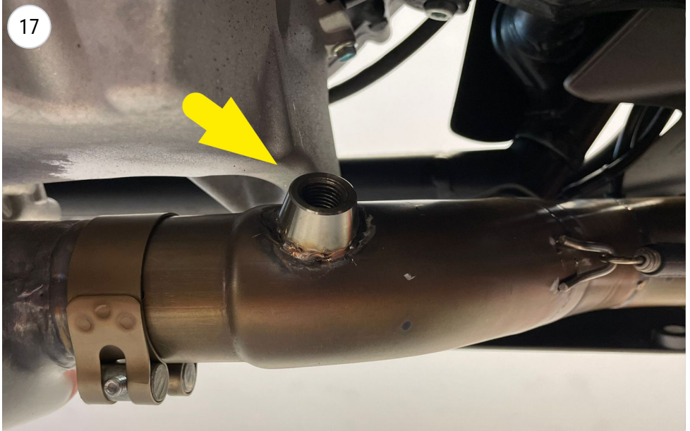
screw the sonda lambda / oxygen sensor
